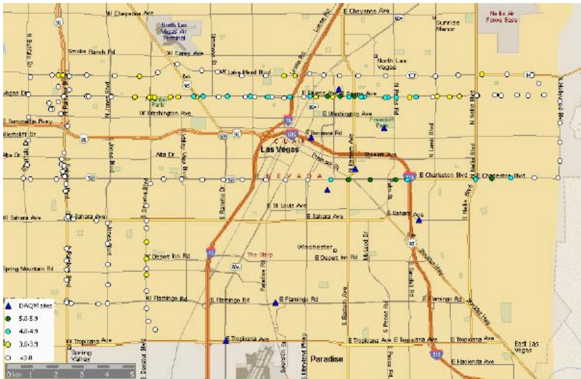
Figure 6-7. Observed CO Concentrations (ppm) During December 16 Evening Period
